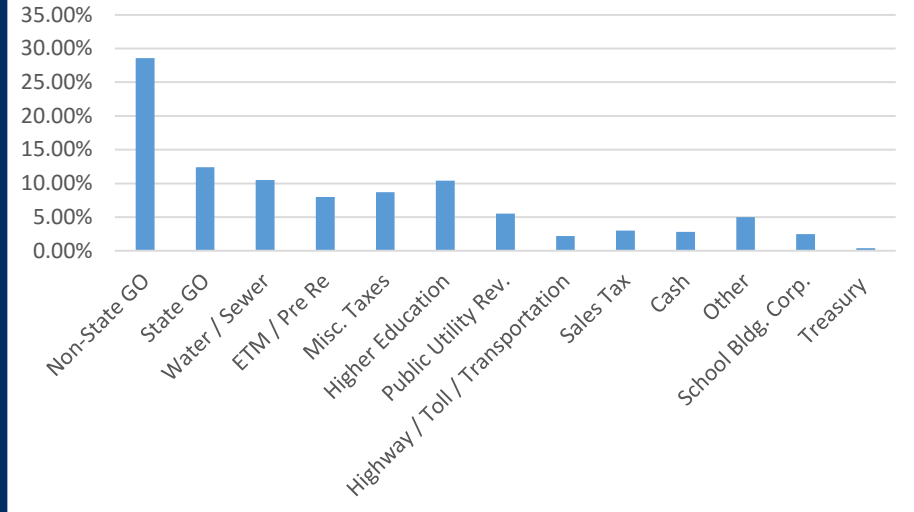
Sector Distribution
