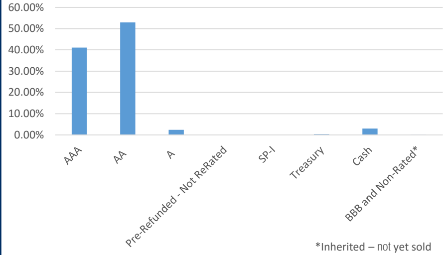
Quality Distribution
